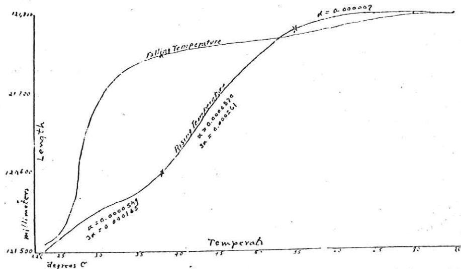
Fig. 8. Linear Expansion of Dental Gutta Percha.
